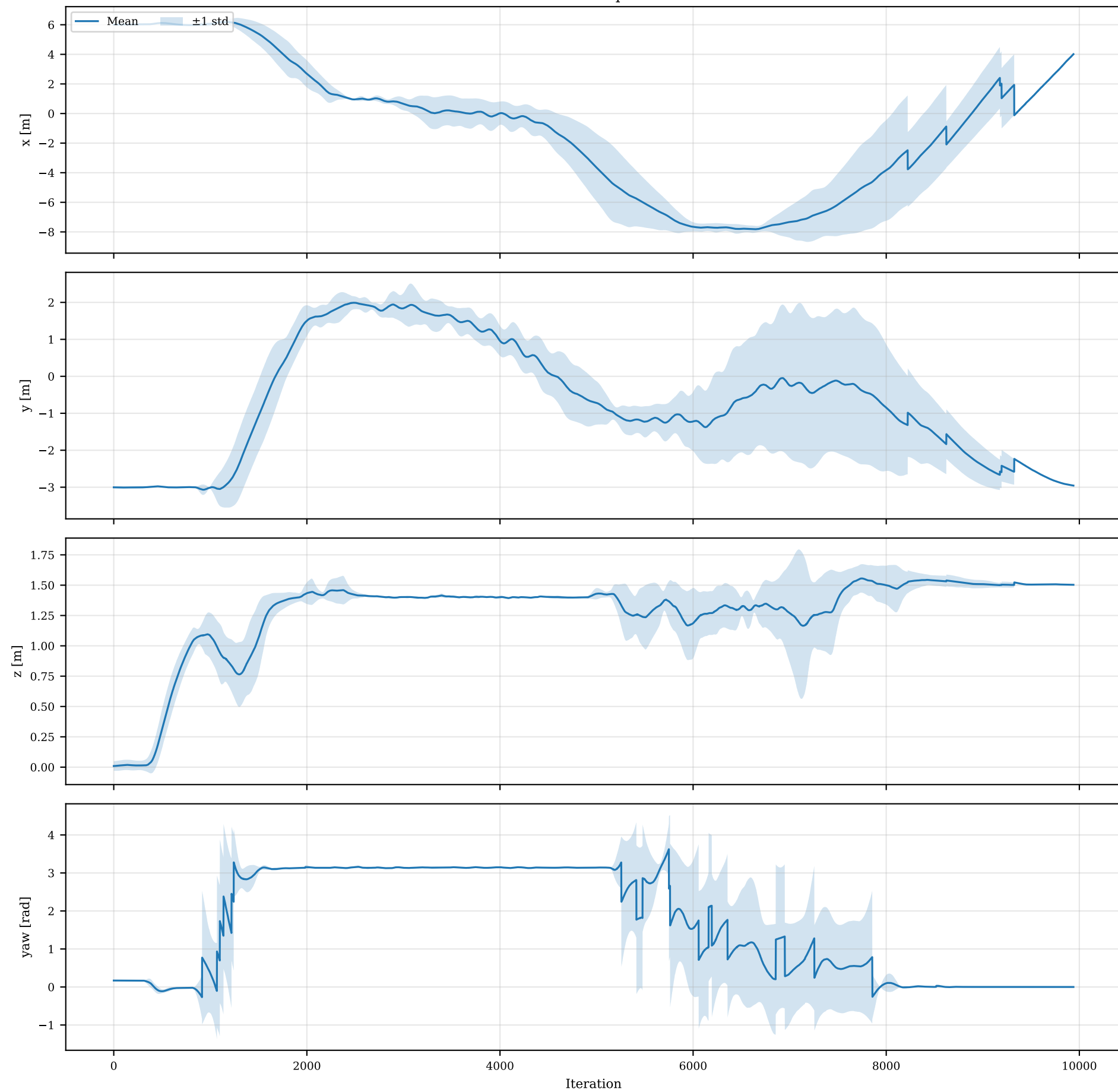
no leader - UAV 29 - Mean position \pm std
